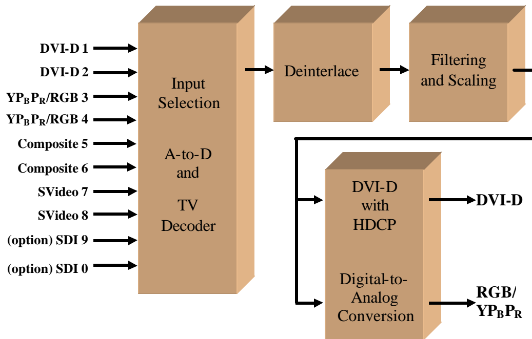
VisionHDP Functional Block Diagram
