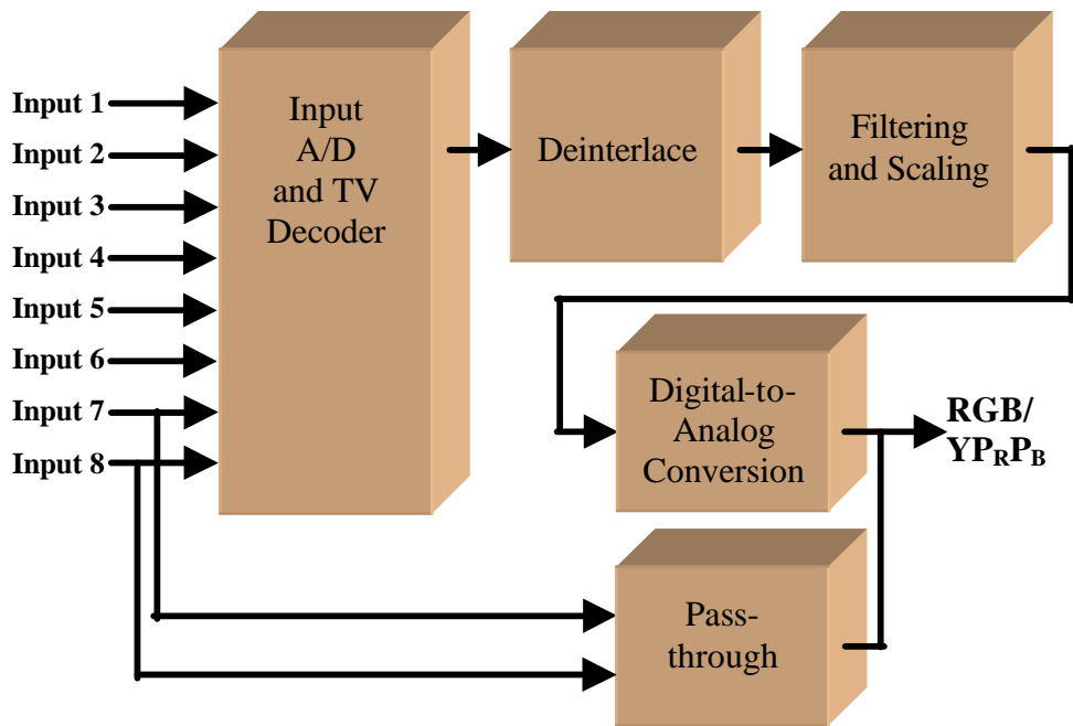
VisionPro Functional Block Diagram
